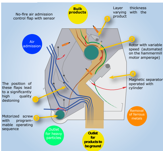
Hammermill feeder principle
